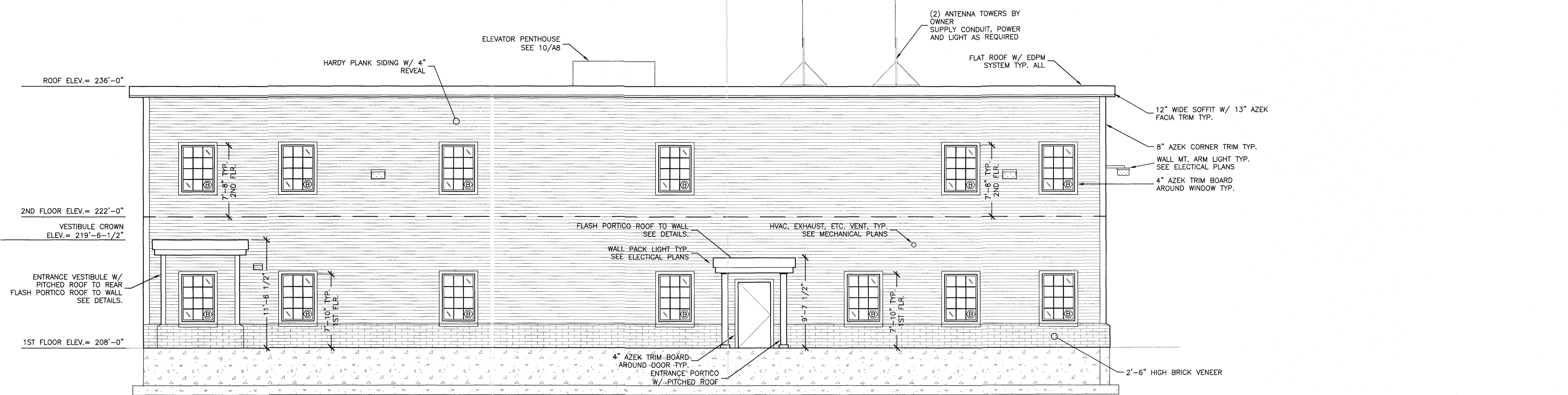
PROPOSED NORTH ELEVATION SCALE: 3/16"=1'-0"
