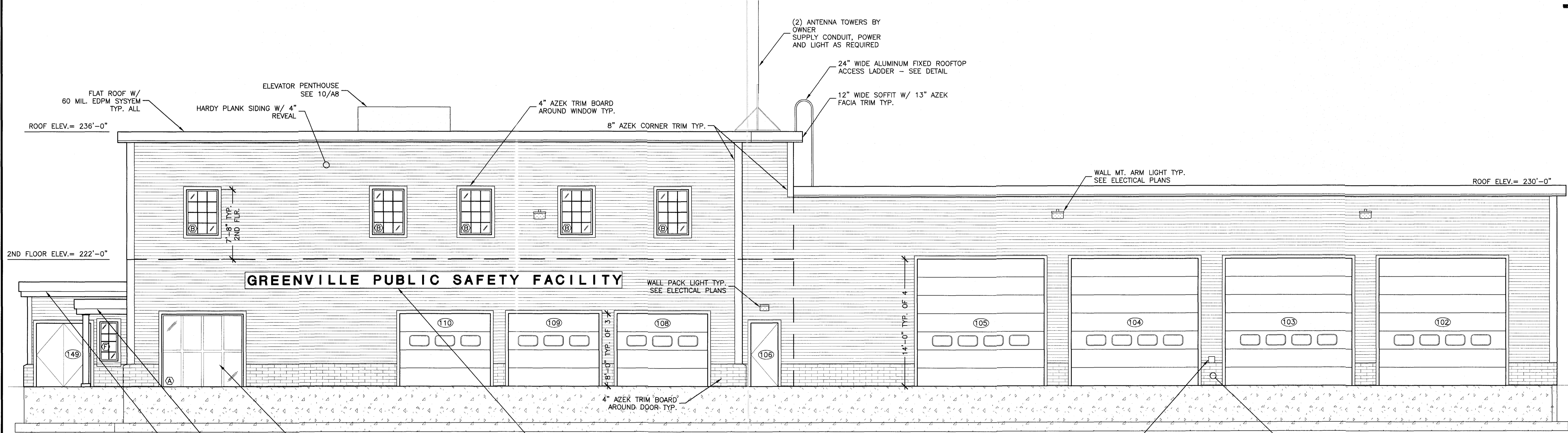
PROPOSED WEST ELEVATION SCALE: 3/16"=1'-0"
