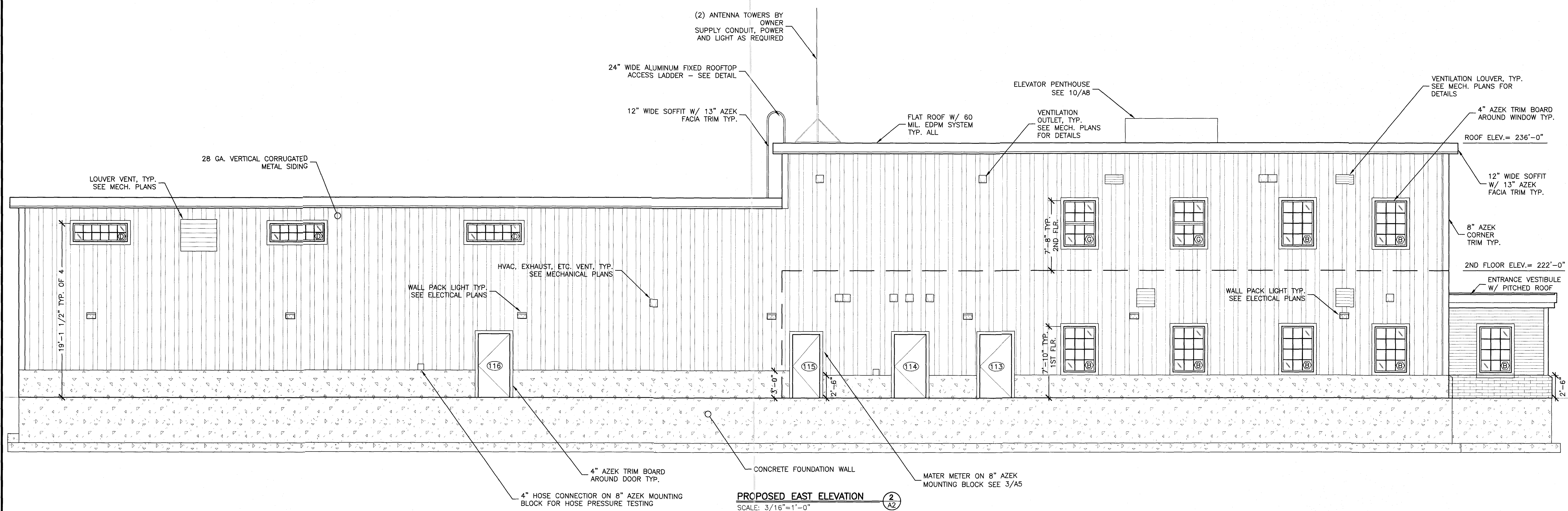
PROPOSED SOUTH ELEVATION SCALE: 3/16"=1'-0" (1 A2)
